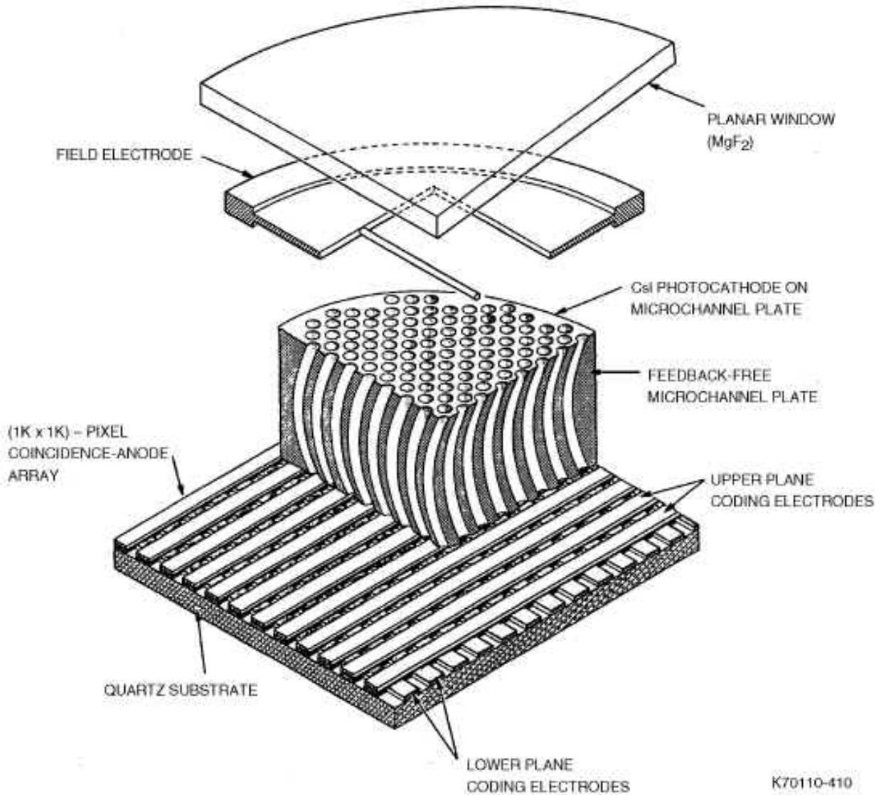
Fig. 4-4 Multi-Anode Microchannel Plate Array (MAMA) detector
