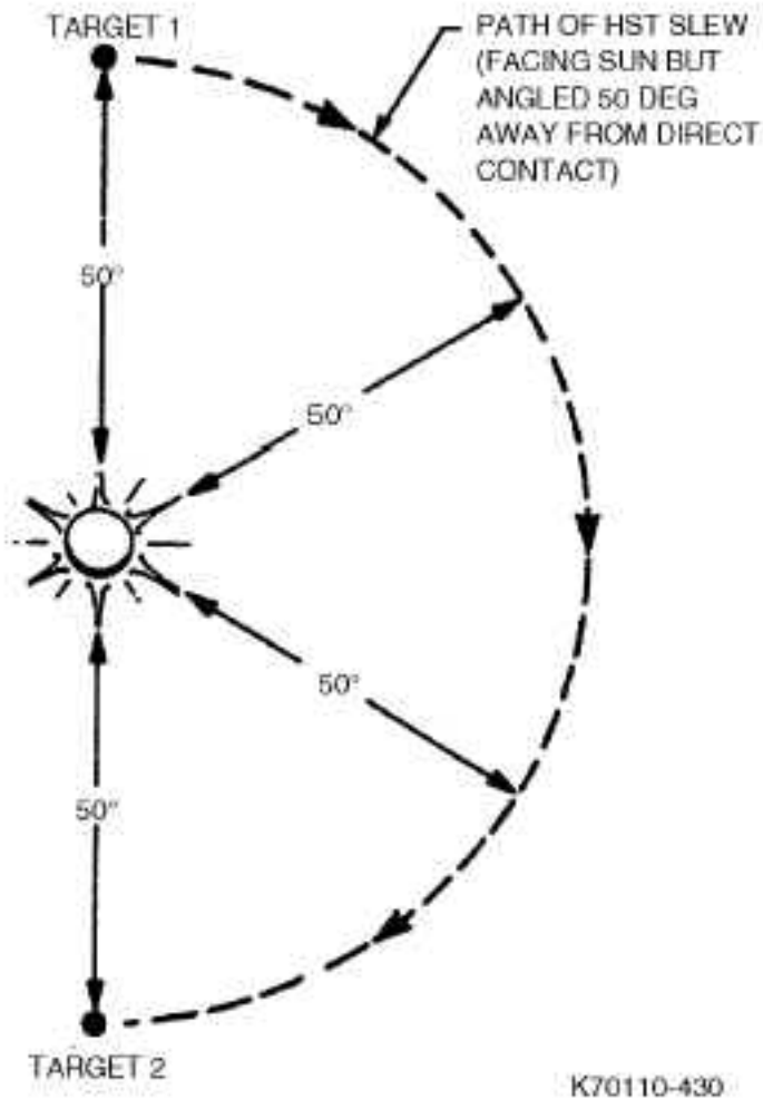
Fig. 6-3 Sun-avoidance maneuver
