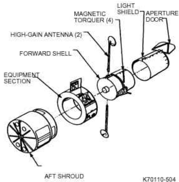
Fig. 5-4 Structural components of Support Systems Module
