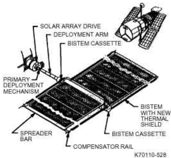
Fig. 5-28 Solar Array wing detail
