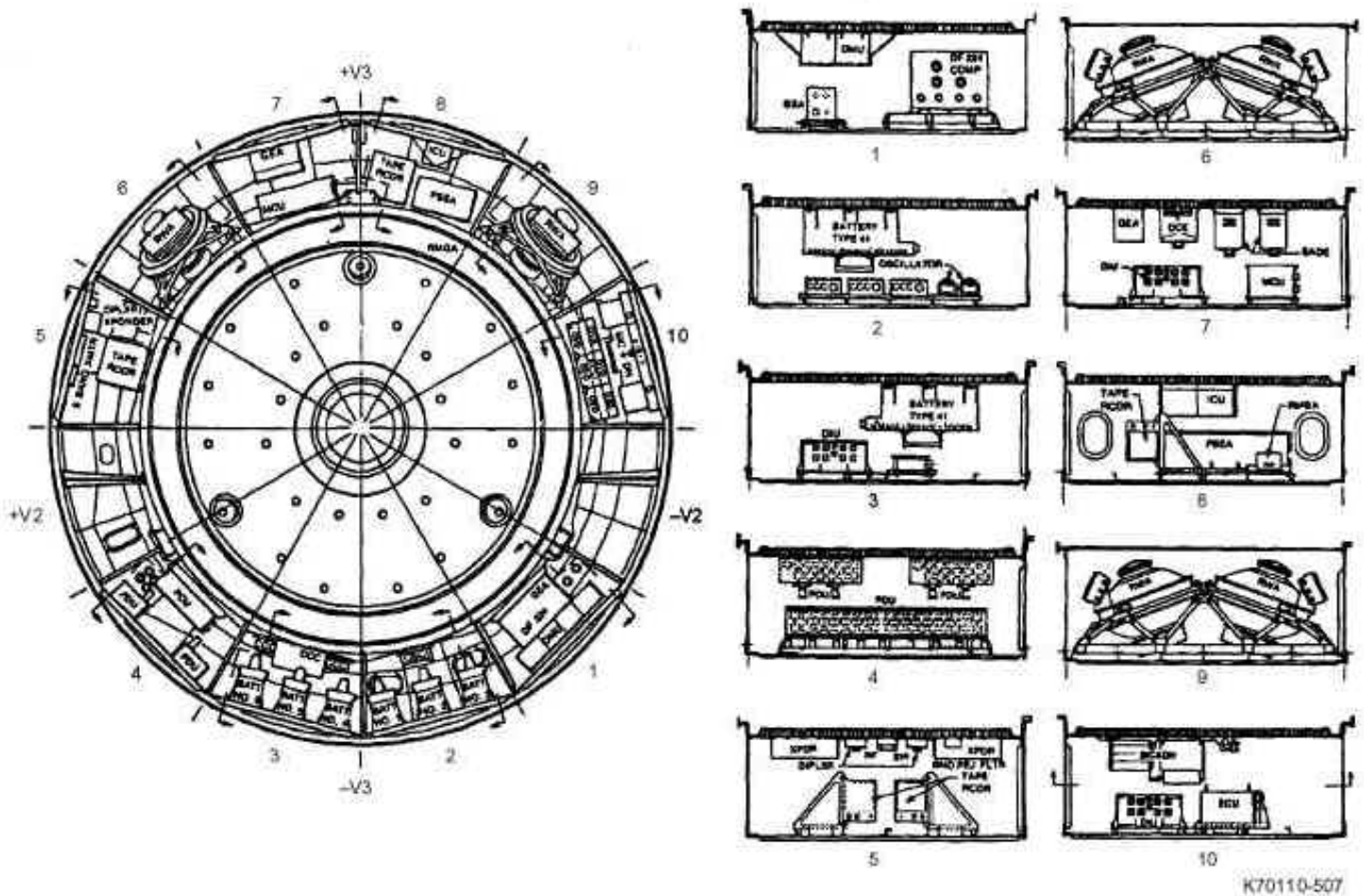
Fig. 5-7. Support Systems Module Equipment Section bays and contents
