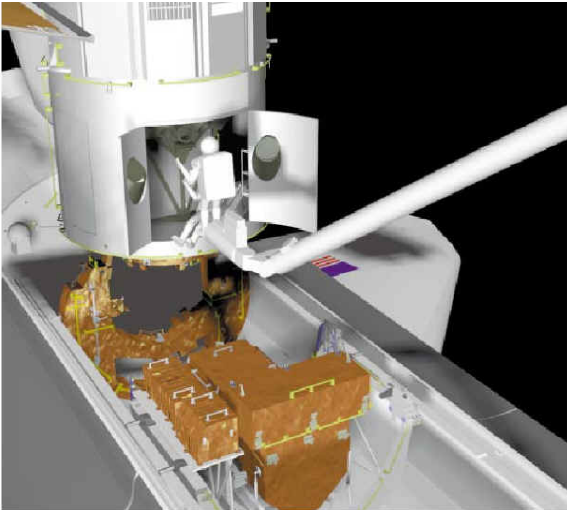
Fig. 2-8 Change-out of Rate Sensor Unit
