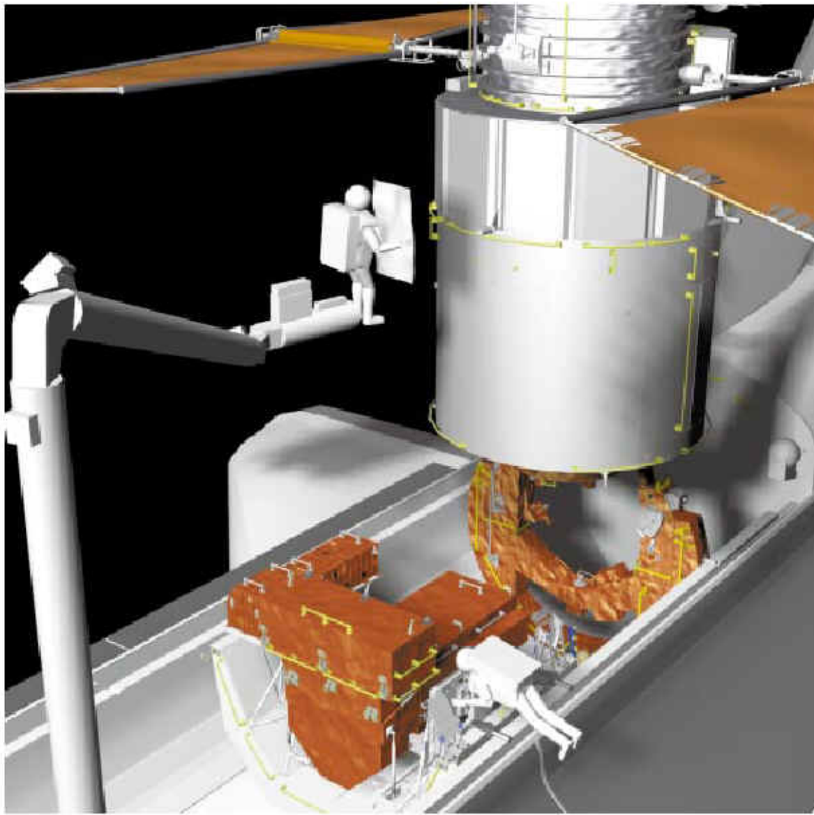
Fig. 2-13 New outer blanket layer installation
