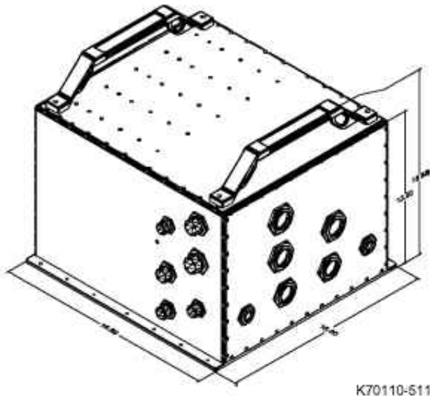
Fig. 5-11 Advanced computer
