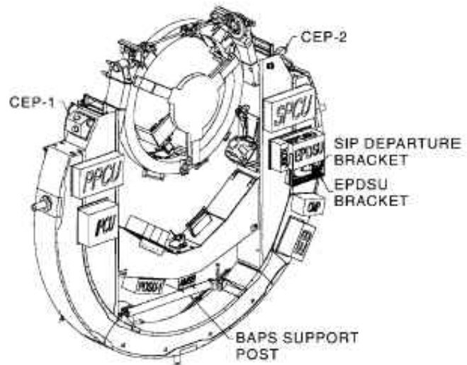
Fig. 5-33 Flight Support System configuration
