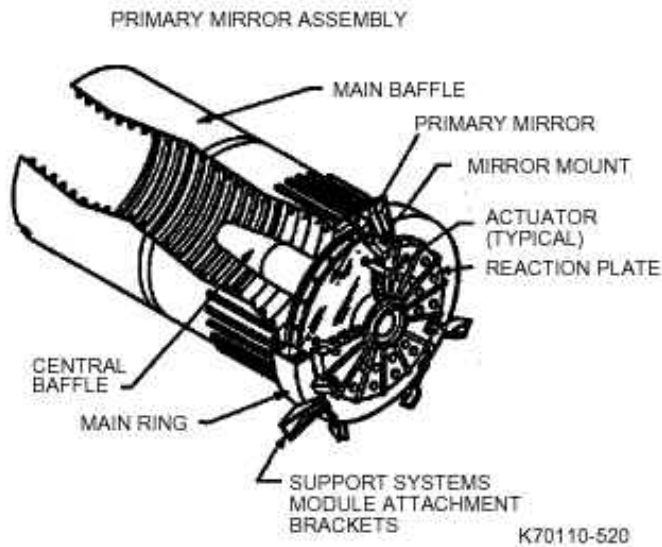
Fig. 5-20 Primary mirror assembly
