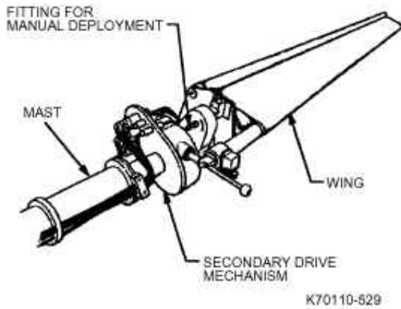
Fig. 5-29 Fitting for Solar Array manual deployment
