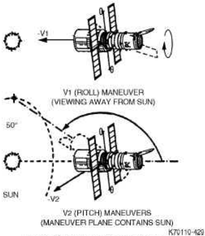
Fig. 6-2 HST single-axis maneuvers
