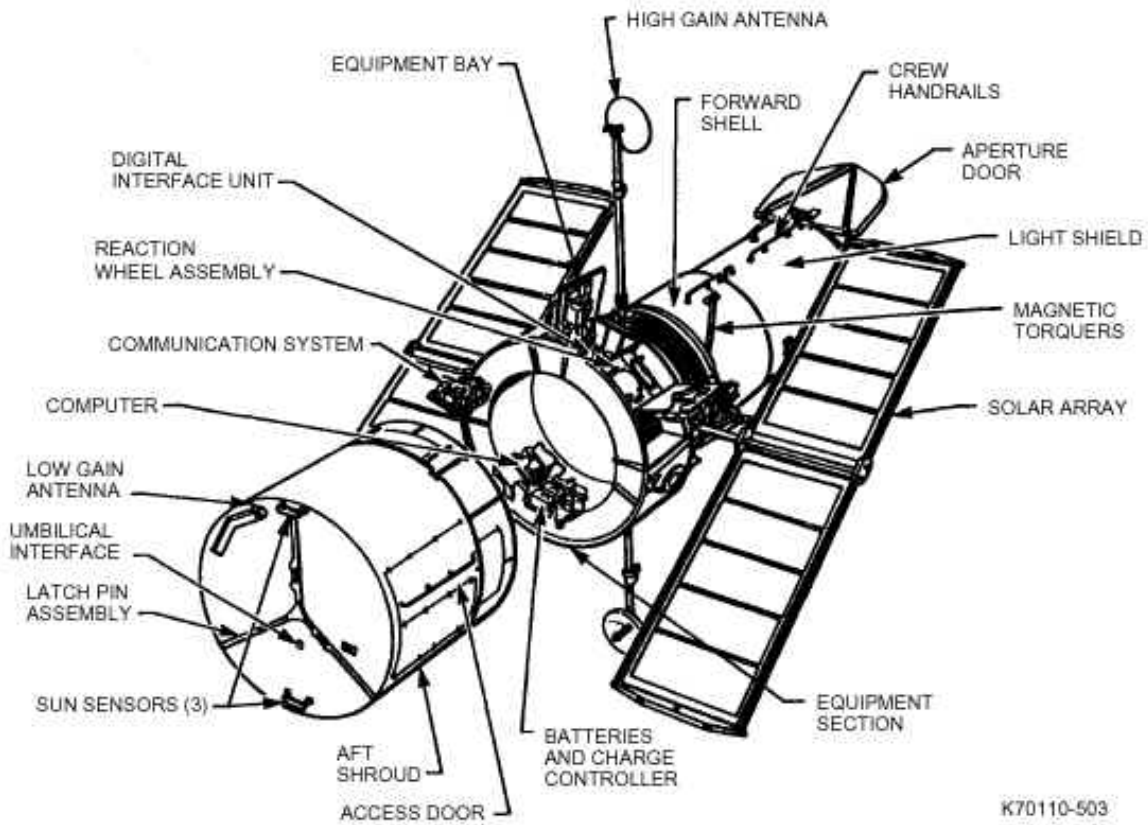
Fig. 5-3 Design features of Support Systems Module
