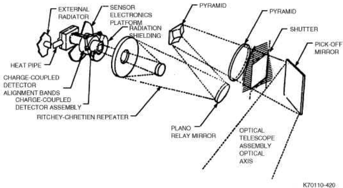
Fig. 4-9 WFPC optics design
