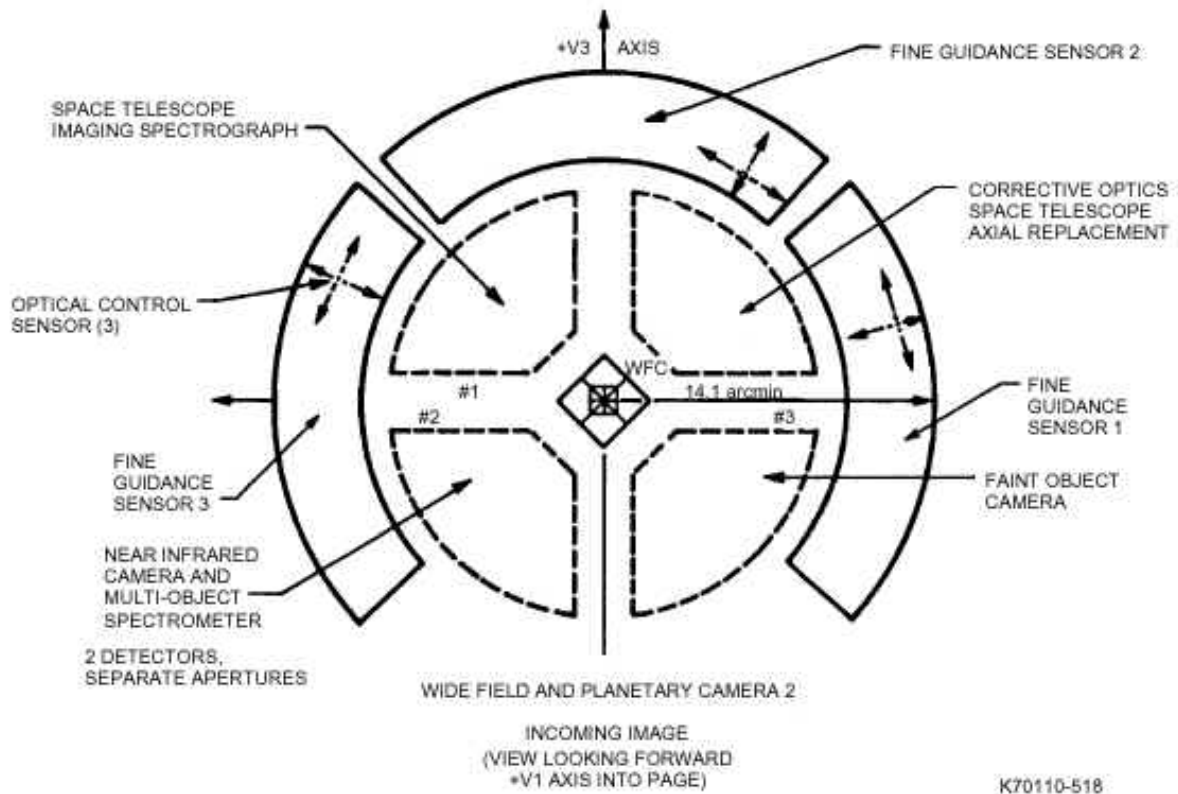
Fig. 5-18 Instrument/sensor field of view
