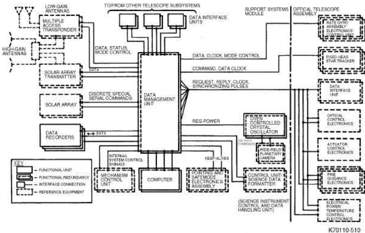
Fig. 5-10 Data Management Subsystem functional block diagram
