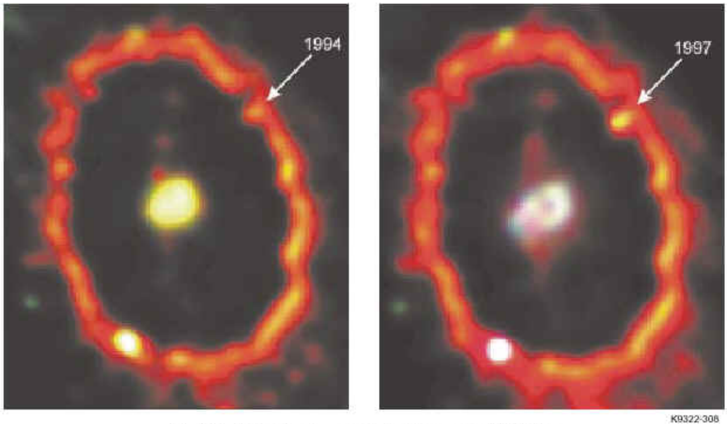
Fig. 3-8 A bright knot appears in the Supernova 1987A Ring.
