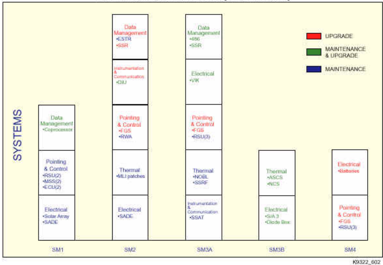
Fig. 7-2 Systems maintained and upgraded during each servicing mission
