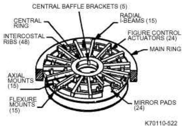
Fig. 5-22 Main ring and reaction plate
