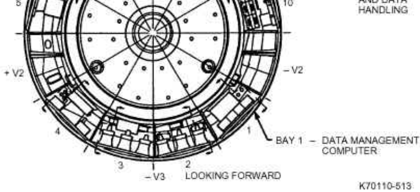
Fig. 5-13 Location of Pointing Control Subsystem equipment
