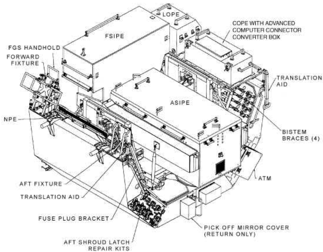
Fig. 2-4 Orbital Replacement Unit Carrier
