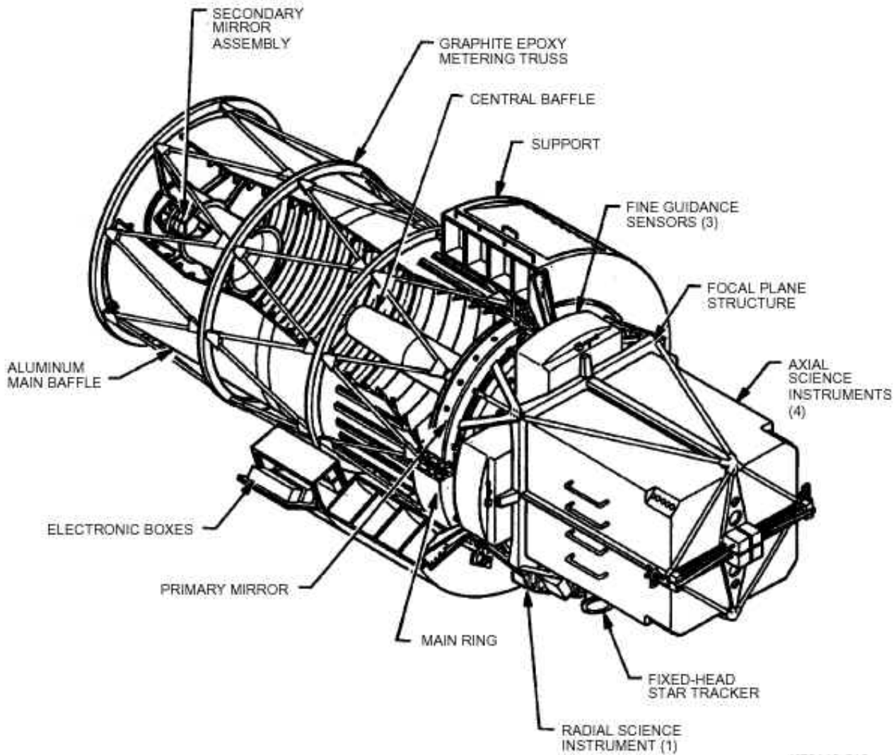
Fig. 5-19 Optical Telescope Assembly components
