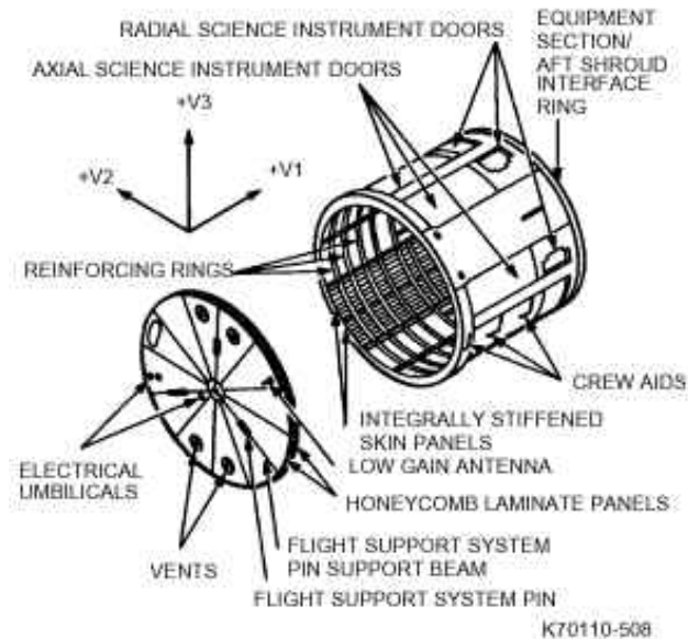
Fig. 5-8 Support Systems Module aft shroud and bulkhead
