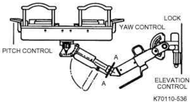
Fig. 5-36 Portable Foot Restraint
