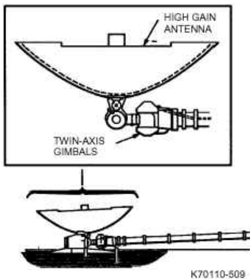
Fig. 5-9 High Gain Antenna
