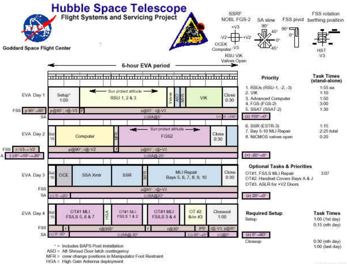
Fig. 2-7 Detailed schedule of extravehicular activities and SA and FSS positions during SM3A
