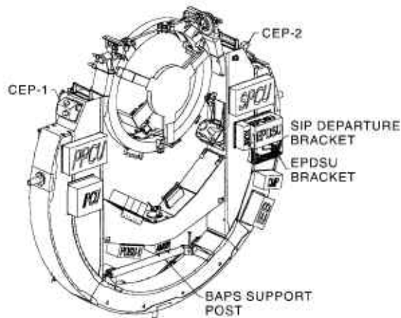
Fig 2-3 Flight Support System configuration
