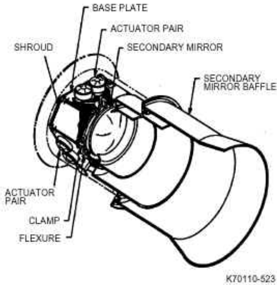
Fig. 5-23 Secondary mirror assembly
