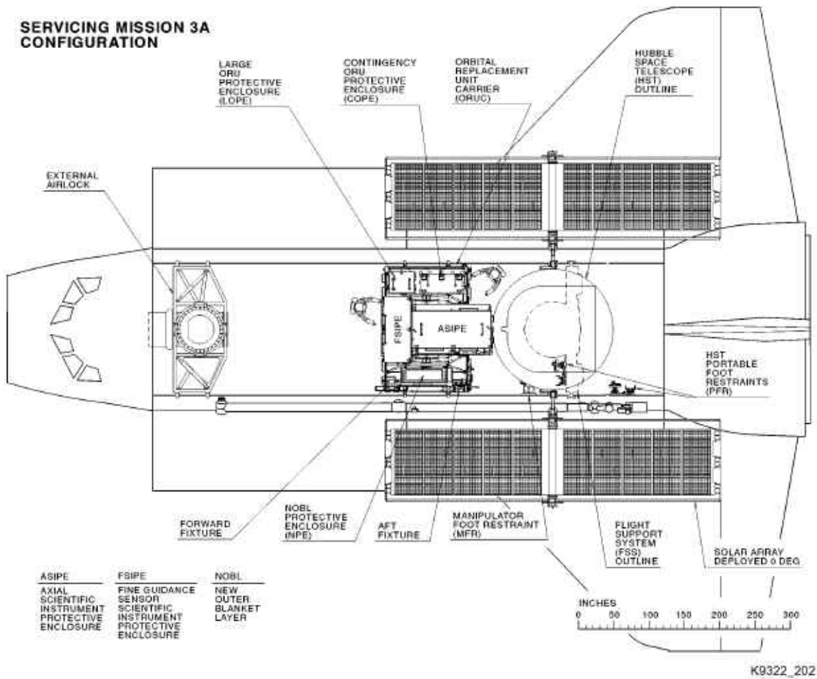
Fig. 2-2 Servicing Mission 3A Payload Bay configuration
