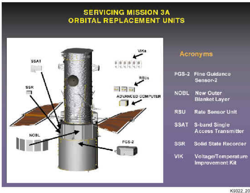
Fig. 2-1 Hubble Space Telescope Servicing Mission 3A Orbital Replacement Units
