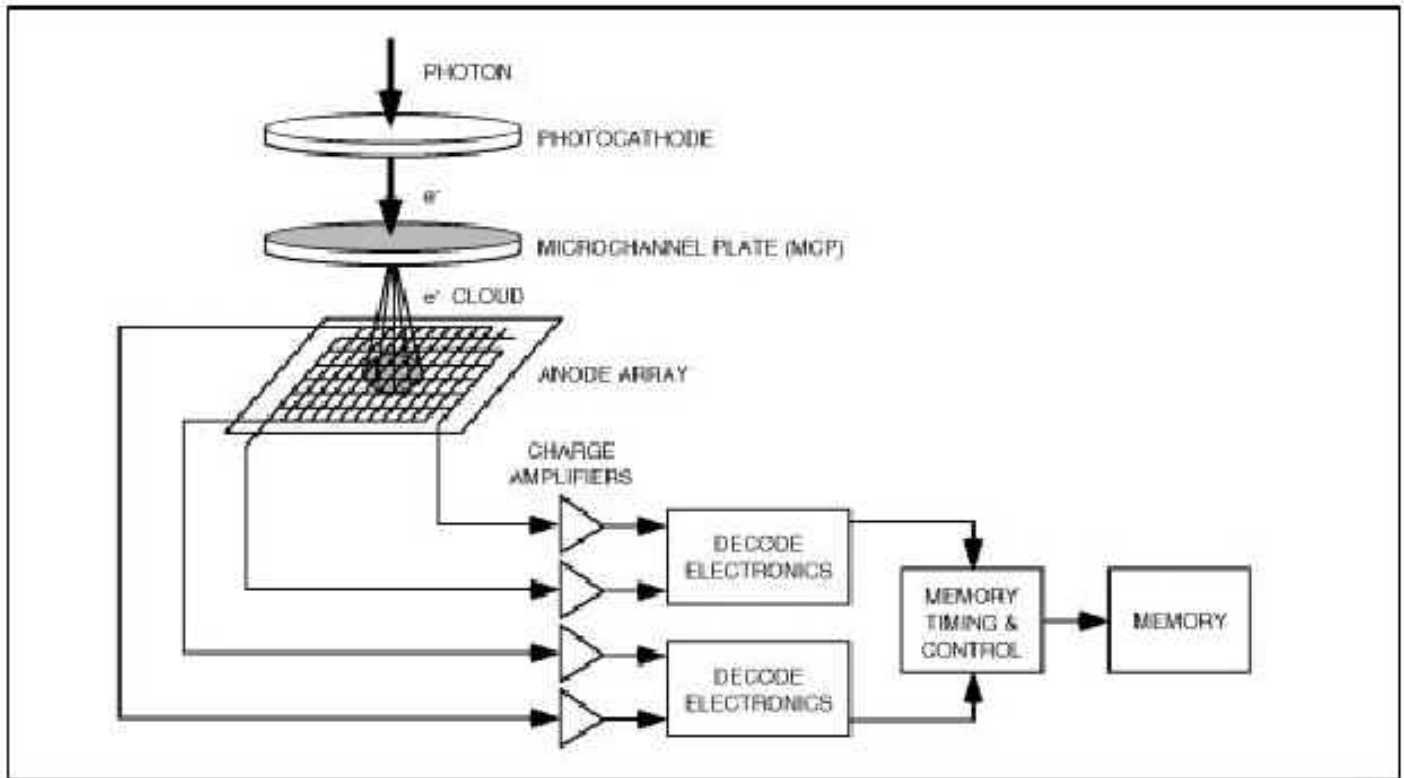
Fig. 4-5 Simplified MAMA system
