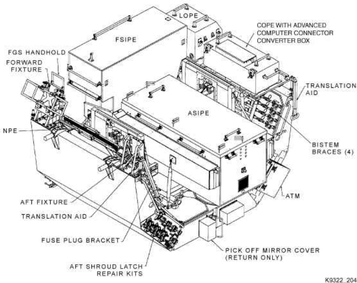
Fig. 5-35 Orbital Replacement Unit Carrier
