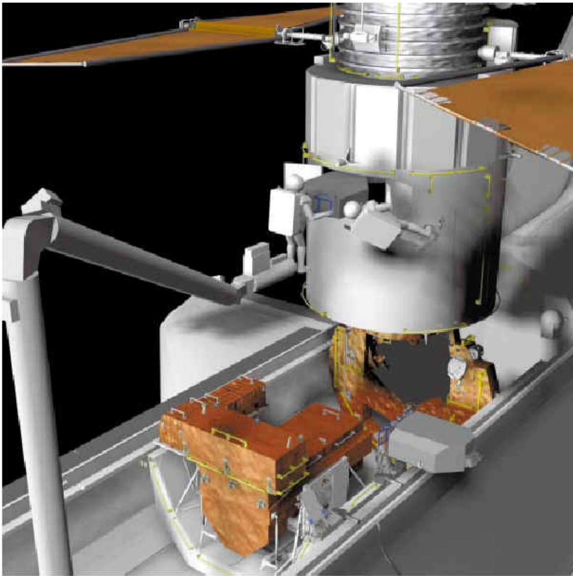
Fig. 2-10 Fine Guidance Sensor change-out
