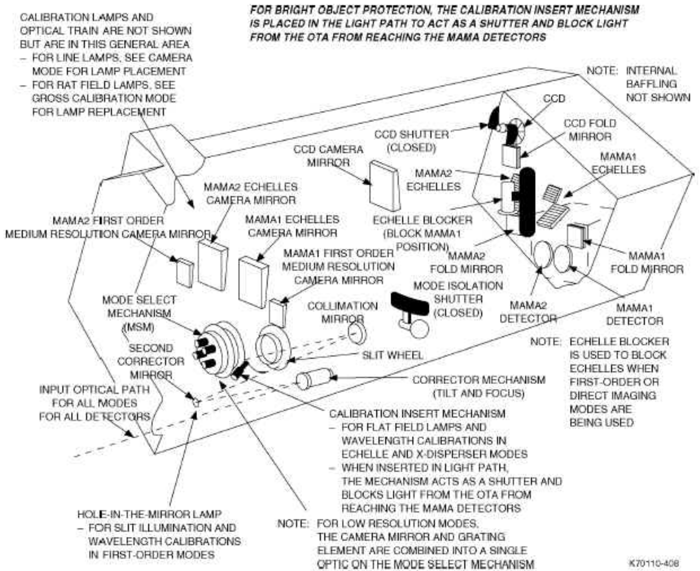
Fig. 4-2 STIS components and detectors
