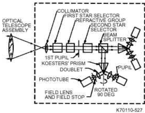
Fig. 5-27 Optical path of Fine Guidance Sensor
