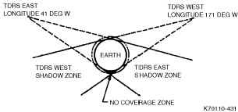
Fig. 6-4 TDRS-HST contact zones
