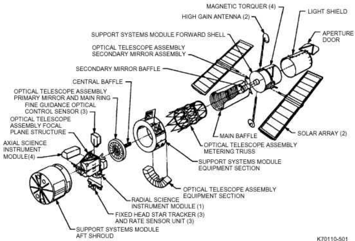
Fig. 5-1 Hubble Space Telescope – exploded view
